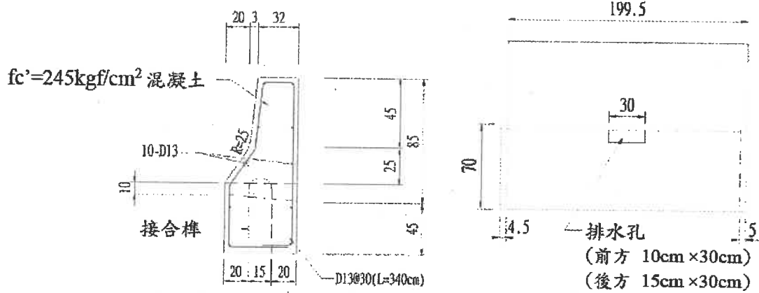
斷面及配筋
